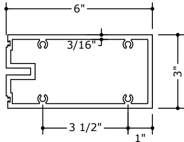
62 HORIZONTAL MULLION
