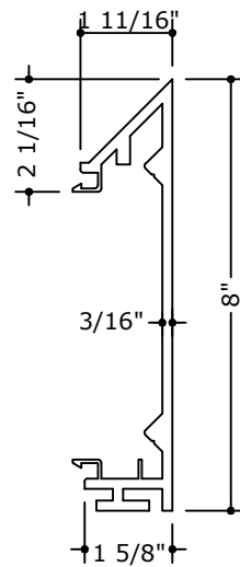
74 90° CORNER MULLION
