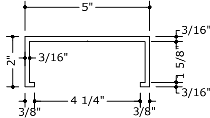
67 SUB-BUCK
