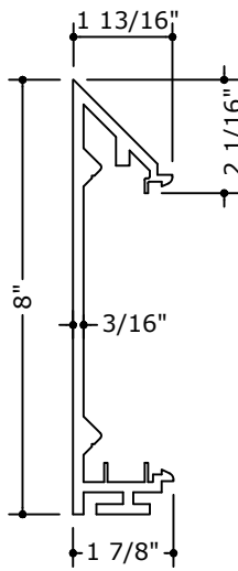
75 90° CORNER MULLION
