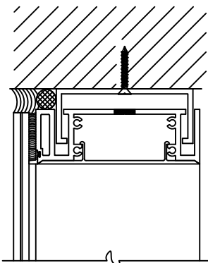
CONDITION 1 HEAD/SILL WITH SUB BUCK (1/8" MAX SHIM)
