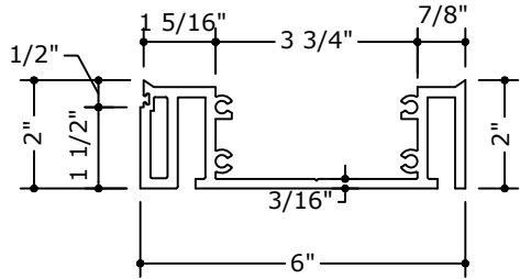
60 HEAD & SILL HORIZONTAL
