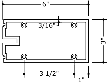
62 HORIZONTAL MULLION
