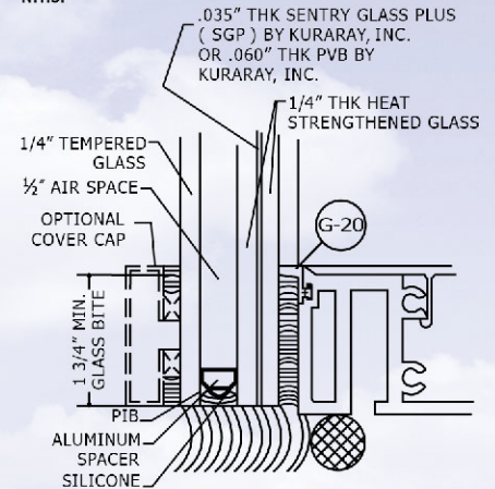
GLASS TYPE A
